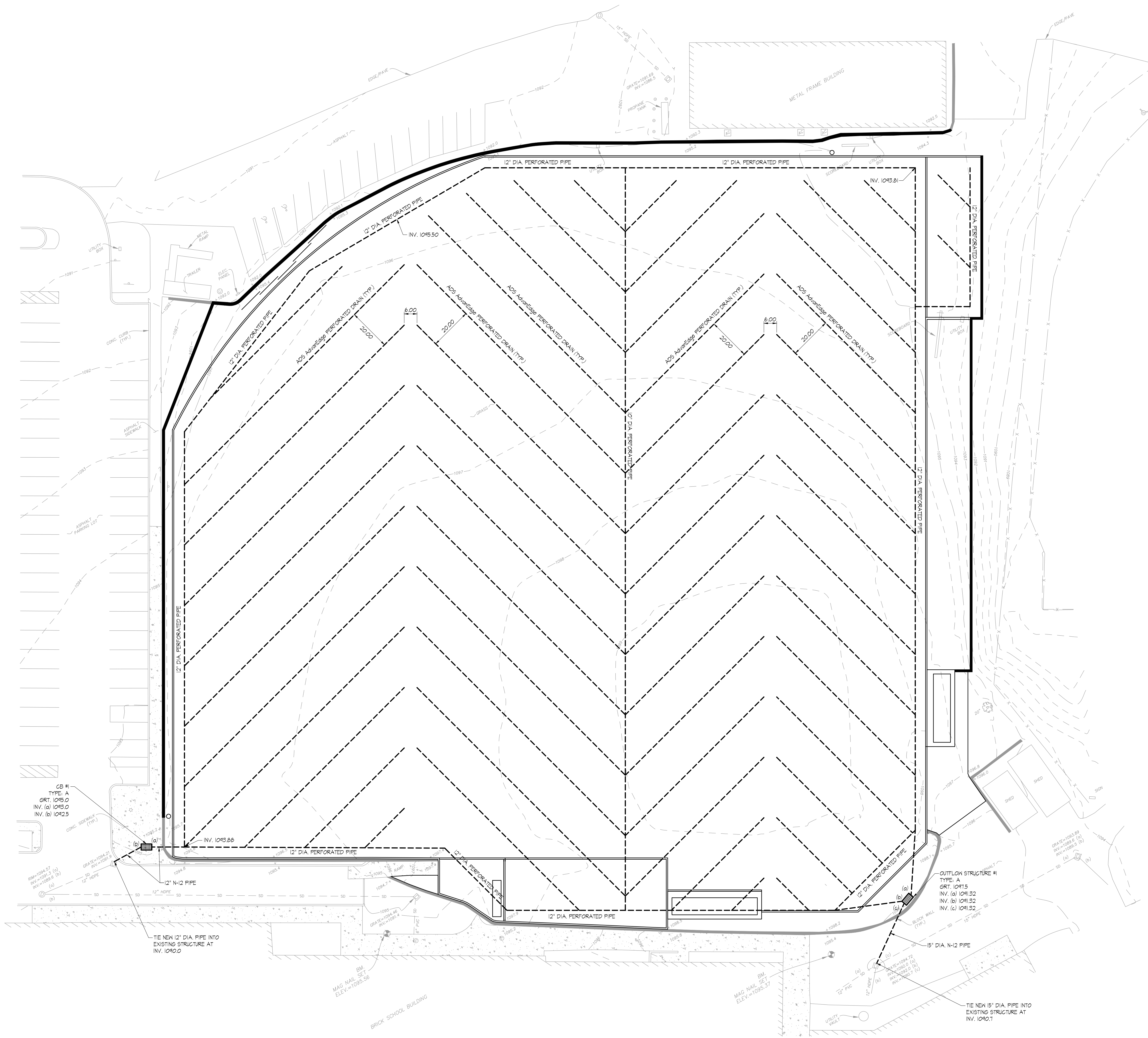
1 STORM WATER DRAINAGE PLAN 1" = 20'-0"
