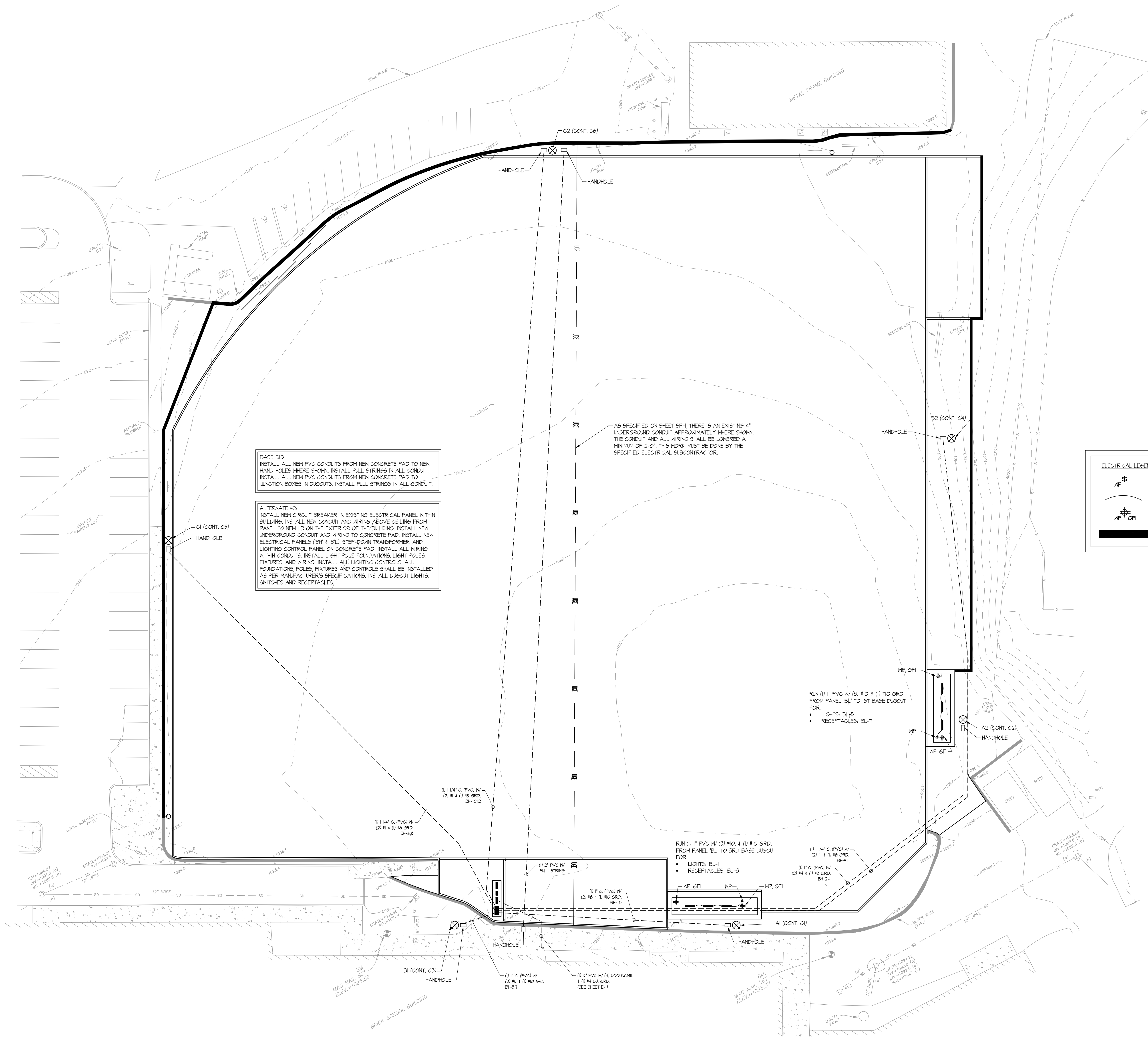
1 ELECTRICAL SITE PLAN 1" = 20'-0"
